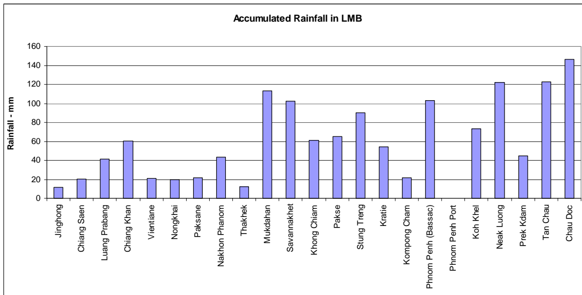
Figure 1: Accumulated Rainfall Distribution over the LMB from 18 th – 25 th September 2017
